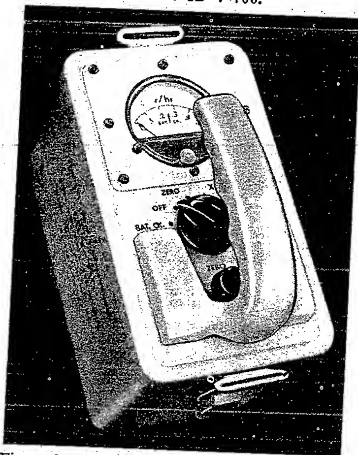
Figure 3.—Medium range gamma survey meter.
